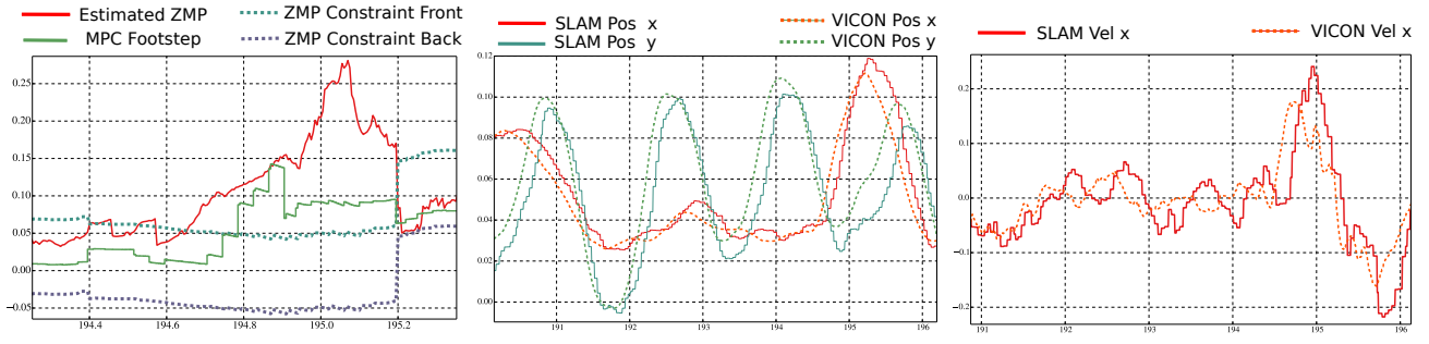
Fig. 5. A strong push forward causes the MPC to step forward to prevent loss of balance. Left - the estimated ZMP from force-sensor measurements is leaving the stability constraint area at time 194.7, the MPC plans a step forward to compensate. Middle - Estimation of the floating base position from SLAM and VICON measurements along the x and y direction. Right - Estimation of the floating base velocity.
