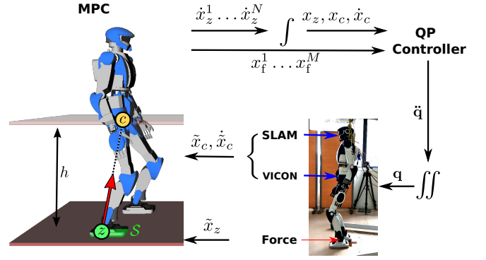
Fig. 2. Overview of the proposed closed-loop MPC. A LIP reduced model is used to represent the dynamics of a humanoid robot walking on flat floor. The pendulum state is estimated from HRP-4 sensors: its CoM position and velocity is obtained with dense visual slam from RGB-D measurements, and its ZMP from force-sensor measurements. This state is used to compute the MPC predictions, i.e. the future ZMP velocities and associated footsteps. Through integration, these references converted to reference position are then tracked by a quadratic programming controller that sends a desired whole-body configuration to the position-controlled robot.
