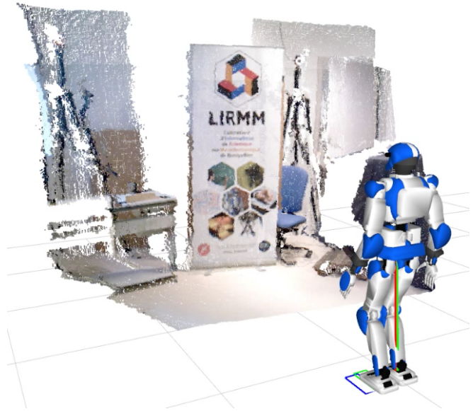
Fig. 1. HRP-4 walking with the proposed closed-loop MPC with dense visual SLAM feedback. The estimated LIP pendulum state obtained from SLAM and force-sensor measurements is shown as a red line going from the ZMP estimate to the robot's CoM. The green line represents the desired pendulum state. Blue and green squares are respectively the desired optimal footstep, and a non-optimal footstep that minimizes changes of the footstep trajectory.
