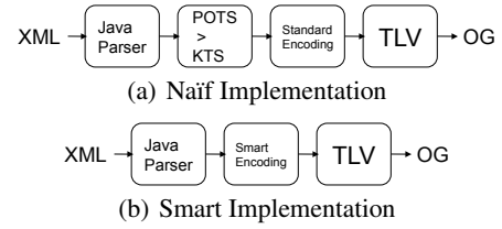
Figure 4: Implementations
