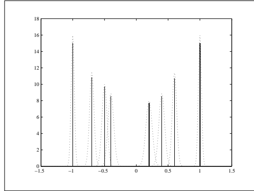
Figure 2. A general overlap distribution function F(q) .
