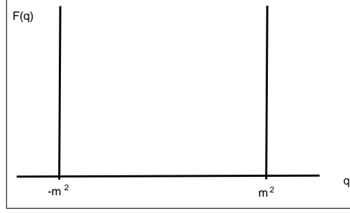
Figure 1. An illustration of the overlap distribution of the Ising model.
