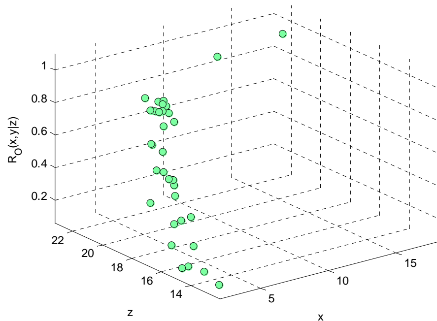
Figure 3. Full frontier ratios against Input Factor (X) and Competition Factor (Z)
