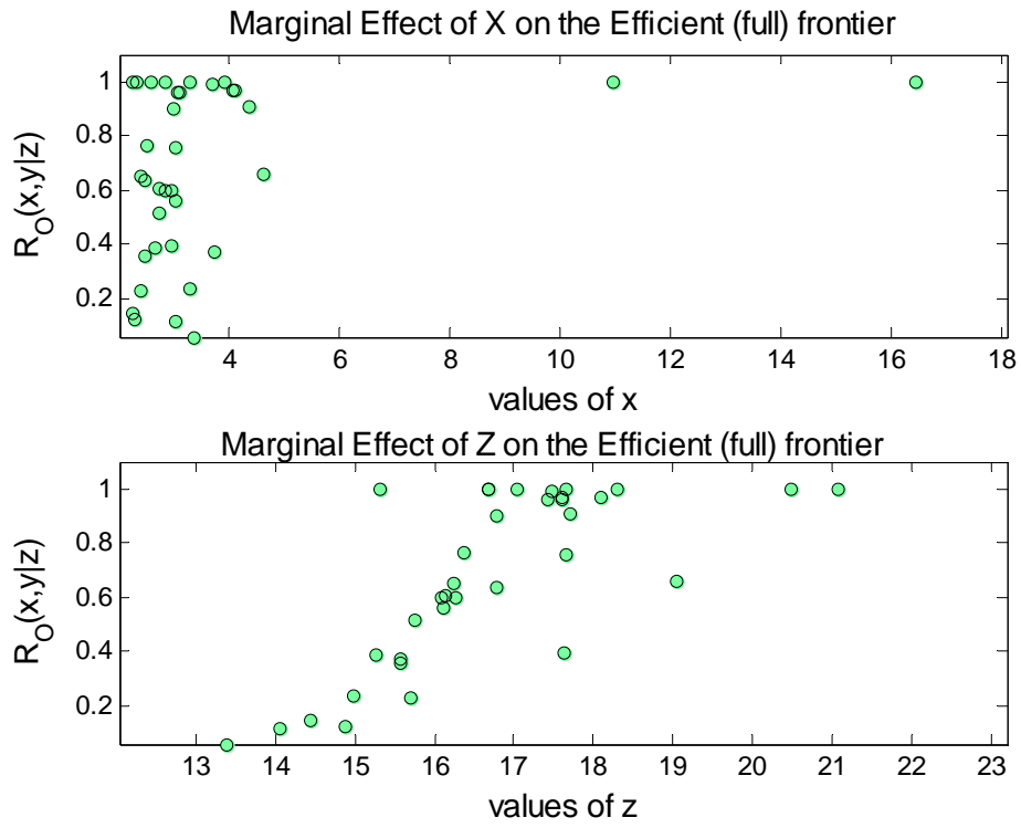
Figure 5. Marginal effect of X and Competition Factor (Z) on the full efficient frontier.
