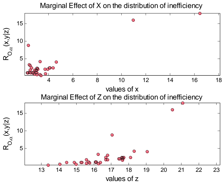
Figure 6. Marginal effect of X and Competition Factor (Z) on the distribution of inefficiency ( \alpha = 0.5 , i.e. median of the distribution of efficiencies)
