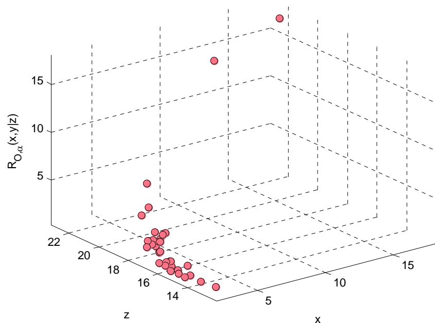
Figure 4. Partial frontier ratios against Input Factor (X) and Competition Factor (Z). ( \alpha = 0.5 , i.e. median of the distribution of efficiencies)
