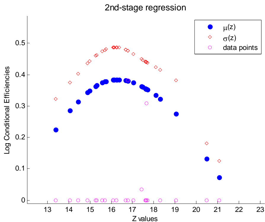
Figure 8. Effect of Competition Index ( Z ) on conditional efficiencies: zoom to highlight the inverse U-shape effect of Z .
