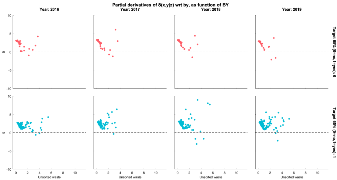
Fig 2 Derivatives of efficiency (one for each municipality) with respect to BY (bad output). Each point represents a municipality.
