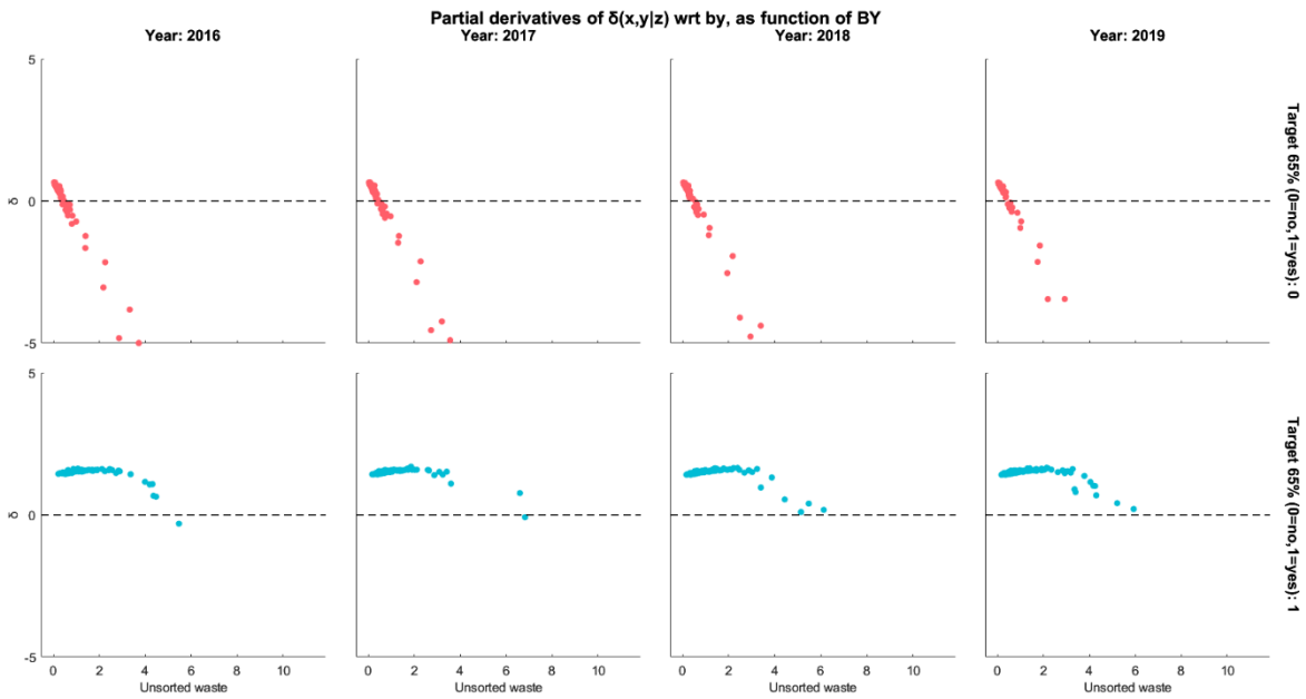
Fig 5 Partial derivatives (one for each municipality) of the efficiency scores conditioned to z =population ( \delta(x,y|z) ) with respect to BY (unsorted waste) as function of BY . Each point represents a municipality.
