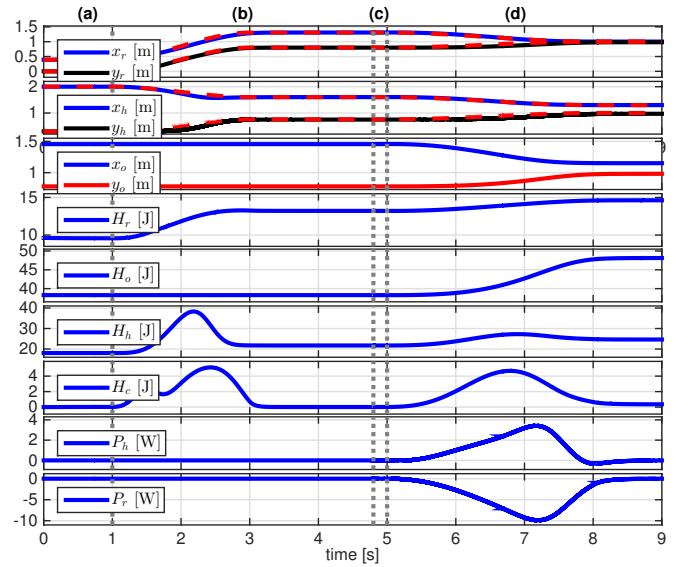
Fig. 3. Evaluation of the energy-based HRC model. In the first two top plots, dashed red lines show the reference positions and solid lines show obtained values. The four phases (a), (b), (c) and (d) are separated by dotted gray lines.
