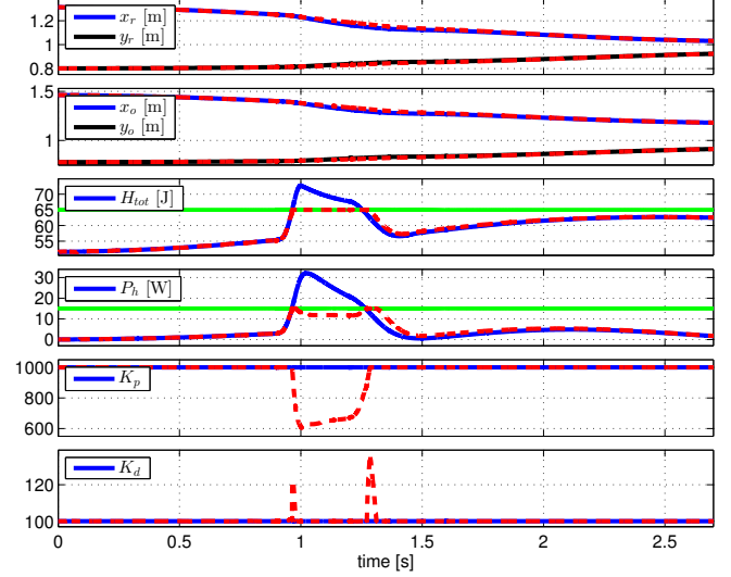
Fig. 4. Validation of energy-based adaptive shared controller. Solid blue and black lines show signals using nominal controller, dashed red lines show signals using safety-enhancing adaptive controller and green lines in the two middle plots show the considered safety thresholds.
