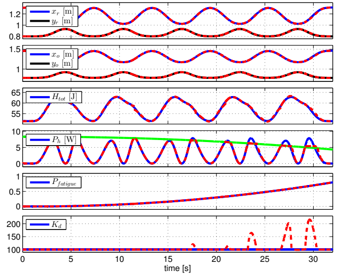
Fig. 5. Validation of energy-based adaptive shared controller for user fatigue reduction. Solid blue and black lines show signals using nominal controller, dashed red lines show signals using the safety-enhancing adaptive controller and the green line in the fourth plot shows the considered adaptive safety threshold.
