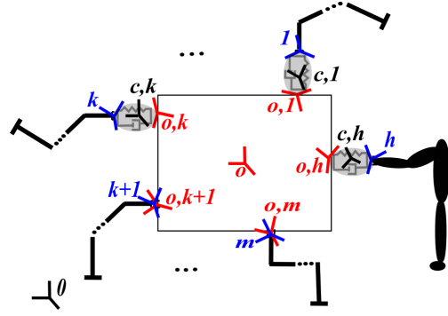
Fig. 1. An example scenario of object transportation by a human and m collaborative robots and possible associated frame definition.
