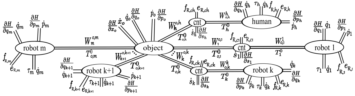
Fig. 2. Port-based representation of collaborative transportation of an object by a human and m robots, each with either rigid contact (direct connection) or compliant contact (represented by cnt).
