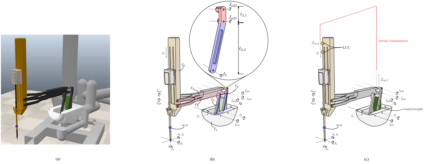
Fig. 1: (a) One of the two PSM arms of the da Vinci Research Kit. The location of the RCM point is also shown in the blue circle. (b) The double parallelgram mechanism highlighted with red and blue squares. Joint axes are highlighted with dashed black lines, with passive joints denoted as J_{p*} . (c) The counterweight modelling solution: the force measured at J_{cw,l} is transmitted to J_{cw,t} , that exerts the same force on the tool through a dedicated loop closure configuration (LCC).
