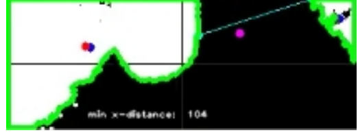
Fig. 4. Distance computation between left and right obstacles. Green curves highlight the contours of the detected obstacles. Blue dots are the corresponding centroids, red dots are the filtered centroids with abscissae x_{l_c} and x_{r_c} . The purple dot is the middle point with abscissa x_m . The horizontal component d_{x,min} of the minimum distance (cyan line) between left and right obstacles is computed on each frame to automatically generate the reference value q_p^* .
