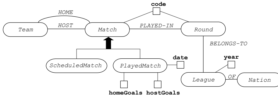
Fig. 2. Diagrammatic representation of the football championship ontology.
