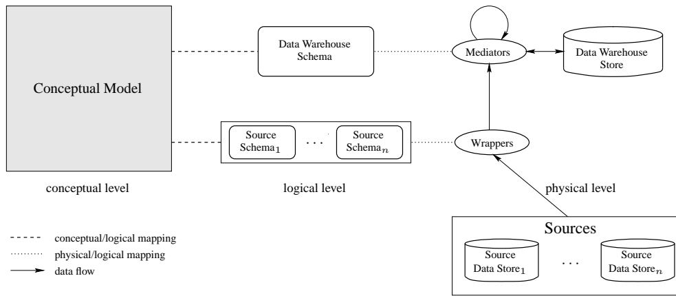
Figure 1: Architecture for Data Integration
