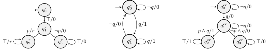
Fig. 4: Machines for Example 5, from left to right: reward machine for (Op, r) , clock machine for \varphi_c , and reward machine for the unlocked-equivalent specification (\varphi_{cr}, r)
