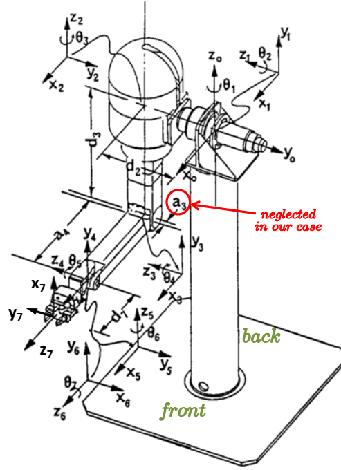
Figure 4: Front view of the DH assignment for the 7R CESAR manipulator (modified from [1]).
